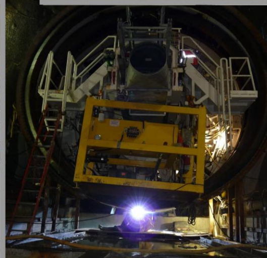
Digging to Times Square, an Inch at a Time New York City and transit officials attended a ceremony Thursday at 25th Street and 11th Avenue, where a 22-foot cutter head was lowered into the ground. The cutter will be mounted on a 100-ton boring machine, which will extend the subway's No. 7 line.
